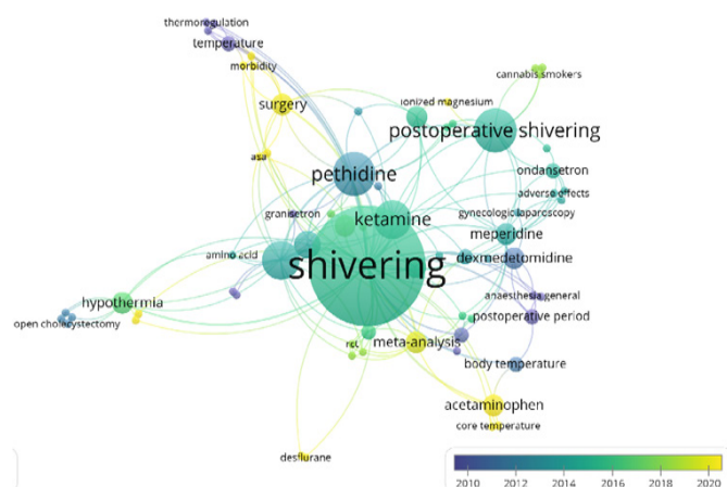
Figure 3. Keyword analysis
